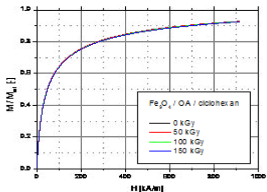
Magnetization curves for non-/ irradiated MF/cyclohexane (OA) (Partner 1 – Politehnica University of Timisoara)
