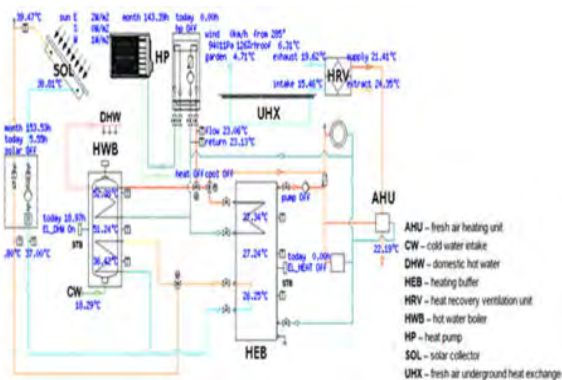
a) Passive house
