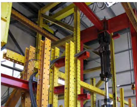
Fig. 1a. Joint specimen after the test
