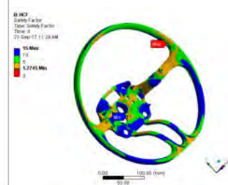
Safety factor under fatigue loading
