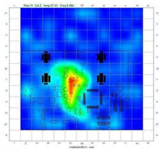
Fig. 3. Near-field scanning
