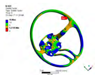
Safety factor under fatigue loading
